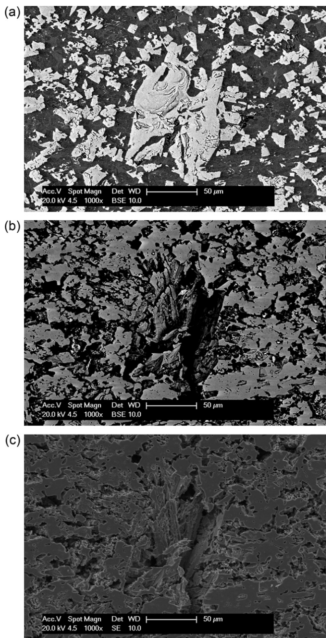
Fig. 9. Surface morphology of bulk crystalline alloy before and after polarisation. (a) BSE image corrosion test (b) BSE image of the same area of the sample after corrosion test showing preferential dissolution of the \text{Mo}_2\text{FeB}_2 (large bright) phase (c) SE image showing preferential dissolution of the \text{Mo}_2\text{FeB}_2 phase.
