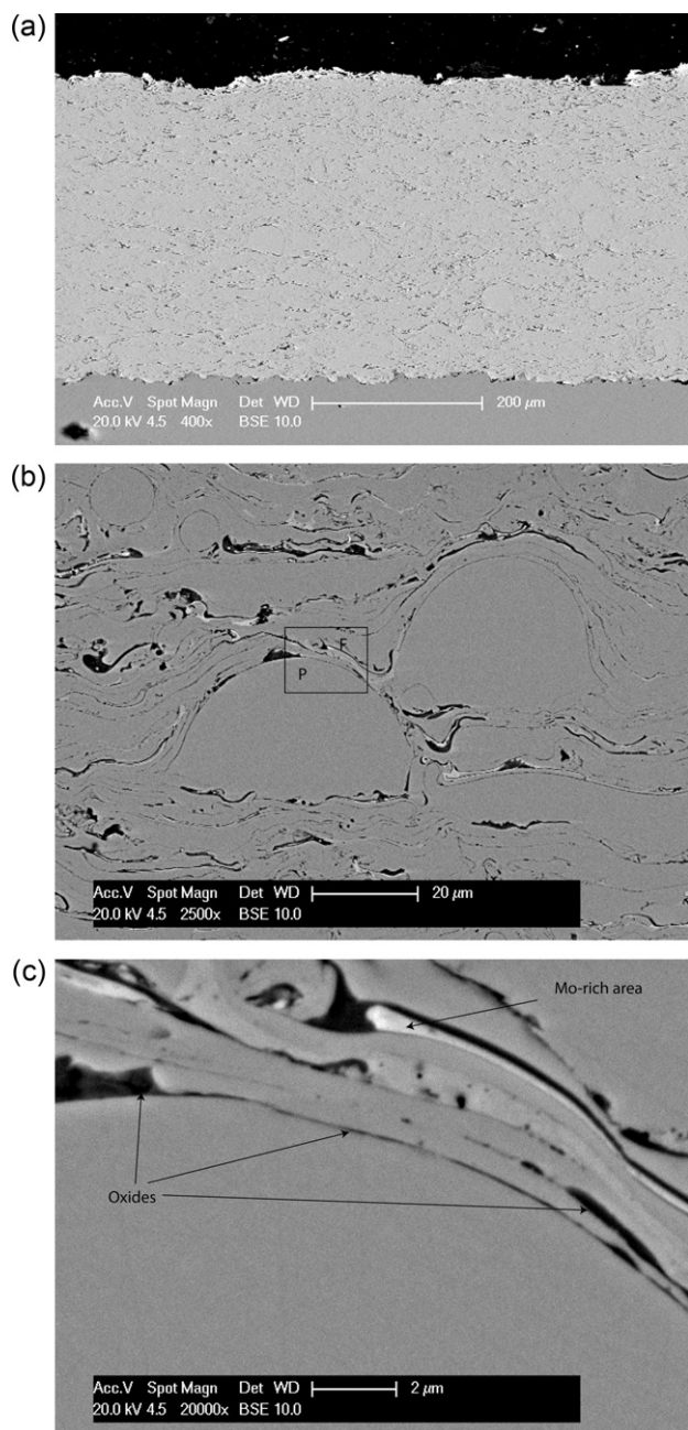
Fig. 5. SEM images of cross-sections of \text{Fe}_{43}\text{Cr}_{16}\text{Mo}_{16}\text{C}_{15}\text{B}_{10} (at%) coated samples (a) full thickness of the coating (b) splat morphology and regions of fully and partially melted material (c) higher magnification of region in the box in b, showing an Mo-rich area and oxides.
