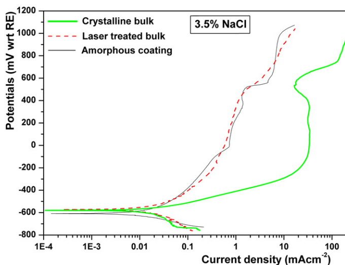
Fig. 8. Potentiodynamic polarisation curves of both crystalline bulk amorphous glass forming alloy and amorphous coating of Fe–Cr–Mo–C–B in 3.5% NaCl.
