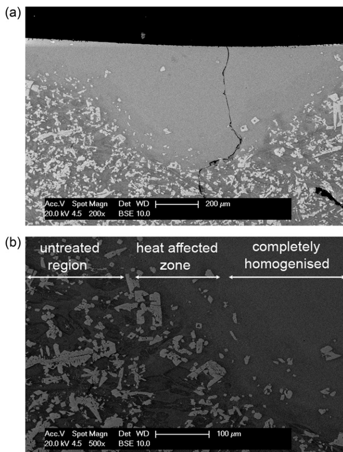
Fig. 4. Back scattered SEM image showing a cross-section of the HVOF feedstock powder.
