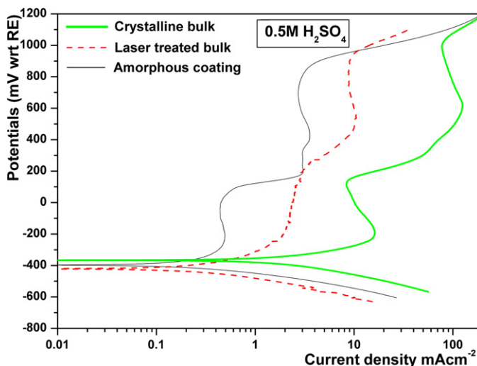
Fig. 7. Potentiodynamic polarisation curves of crystalline glass forming alloy, amorphous GF bulk alloy and amorphous coating Fe–Cr–Mo–C–B in 0.5 M \text{H}_2\text{SO}_4 .
