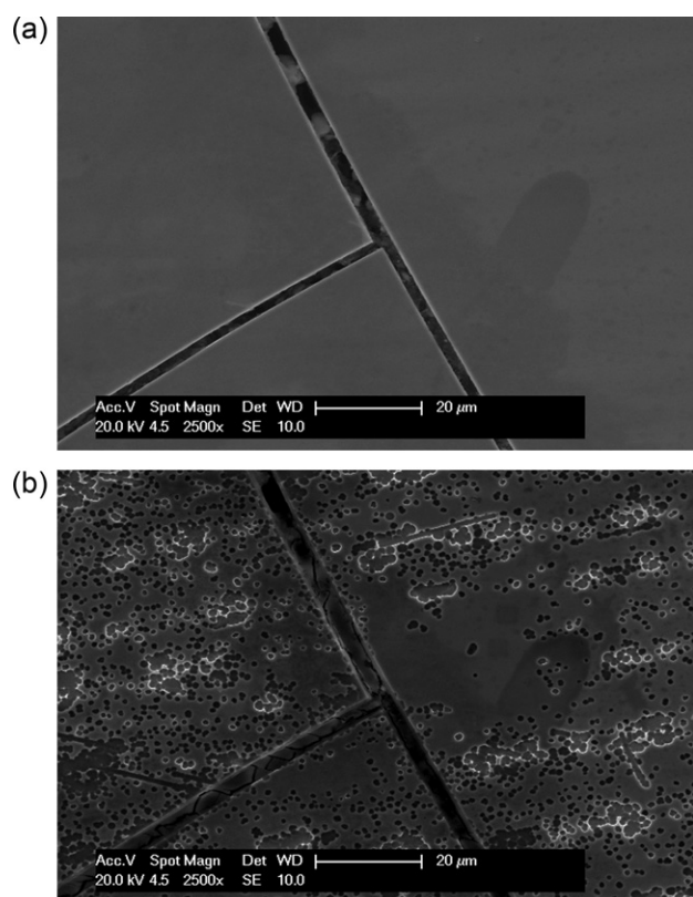
Fig. 11. Surface morphology of a selected area of the laser treated amorphous sample before and after polarisation. (a) SE image before corrosion test in acid (b) SE image of the same area after corrosion test in acid.
