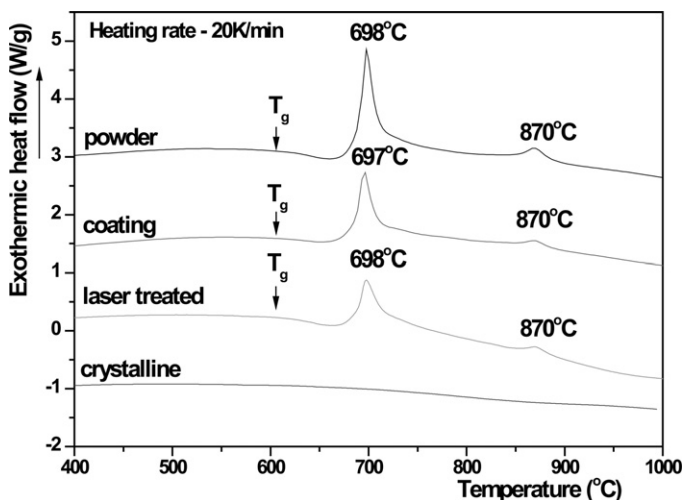
Fig. 6. DSC traces for powder, coating, laser treated and crystalline bulk forms of the alloy.
