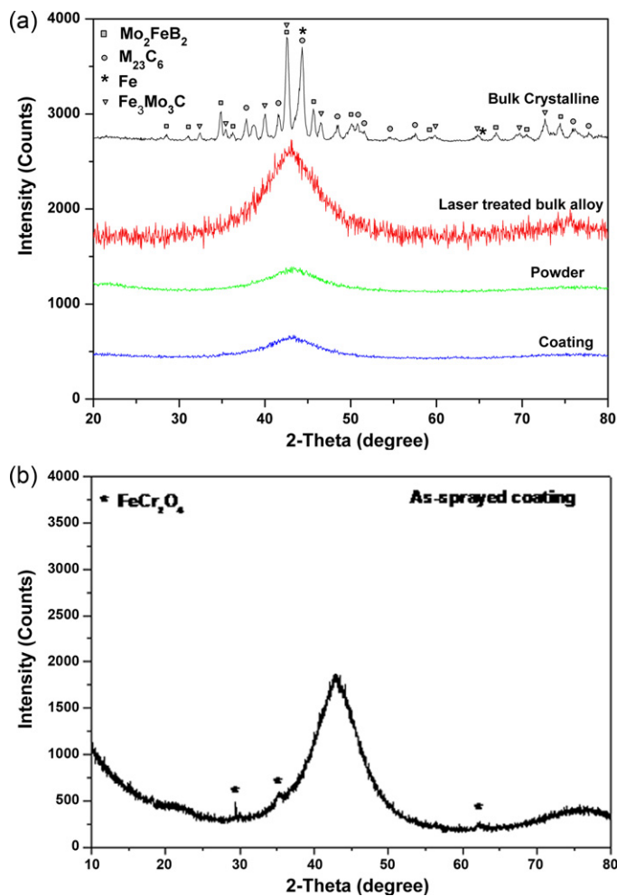
Fig. 2. (a) Comparison of XRD scans of \text{Fe}_{43}\text{Cr}_{16}\text{Mo}_{16}\text{C}_{15}\text{B}_{10} (at%) alloy showing peaks of different phases in the crystalline glass forming alloy and halo peaks in amorphous laser treated bulk alloy and coating, (b) oxide peaks detected for the HVOF coating.
