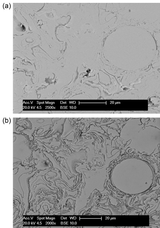
Fig. 10. Surface morphology of amorphous sprayed coating samples before and after polarisation in BSE mode (a) before corrosion (b) after polarisation in 0.5 M \text{H}_2\text{SO}_4 showing clearly the origin of corrosion at the melted and resolidified region around the splat.
