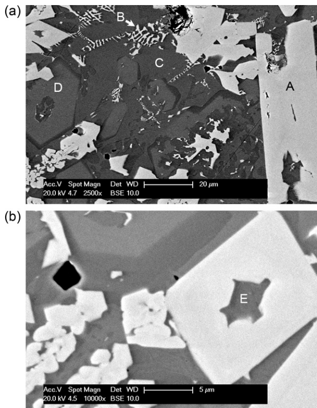
Fig. 1. Back scattered SEM image showing a plan view of the as-cast glass forming alloy (a) Four different phases (A–D) are labelled; (b) higher magnification image showing a fifth phase (E).
